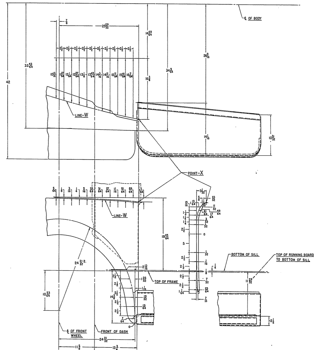
BODY BUILDERS LAYOUT R, RA T, TA V, VA FRONT FENDER AND RUNNING BOARD
